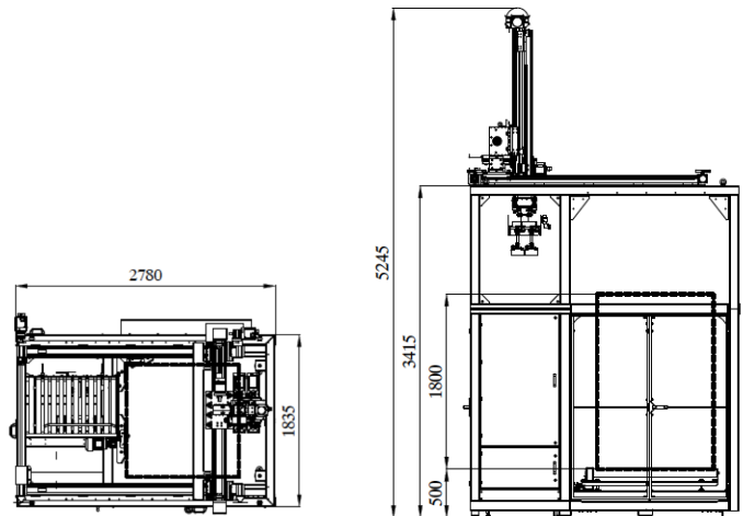
Configuration for 1,800 mm height pallet on 500 mm conveyor. Check sizes for other options.
